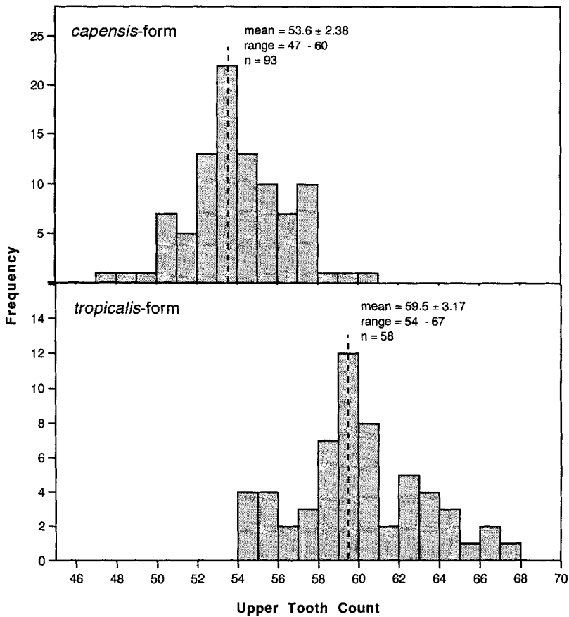
Figure 3. Histogram of upper tooth counts for capensis -form and tropicalis -form specimens.
