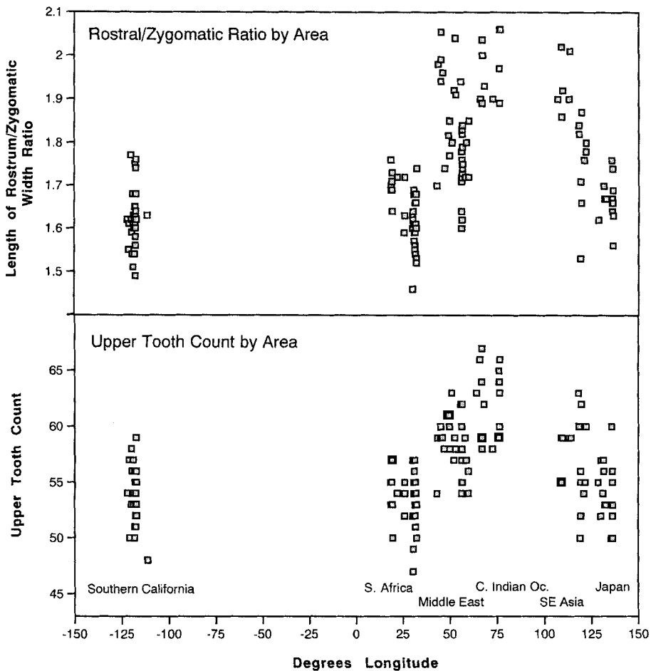
Figure 7. Scatterplot of skull dimensions and upper tooth counts plotted against locality of specimen in degrees longitude.
