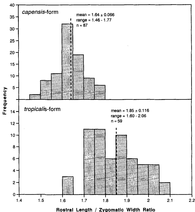
Figure 4. Histogram of rostral length/zygomatic width ratios for capensis -form and tropicalis -form specimens.
